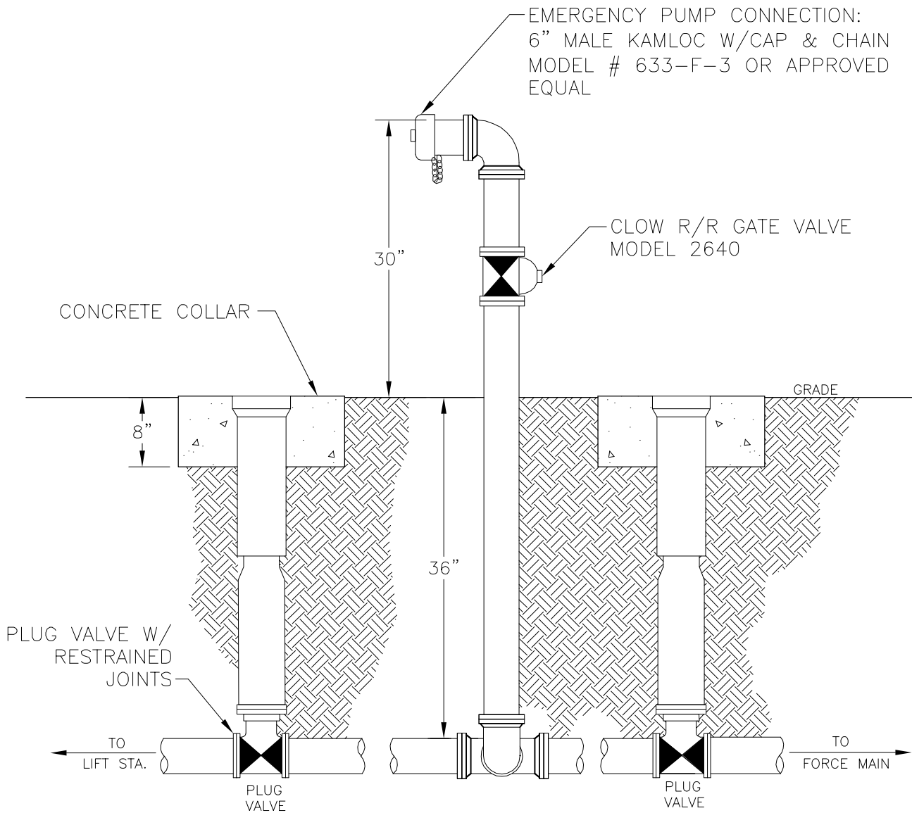
ELEVATION VIEW
